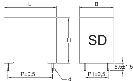
4 terminals execution
